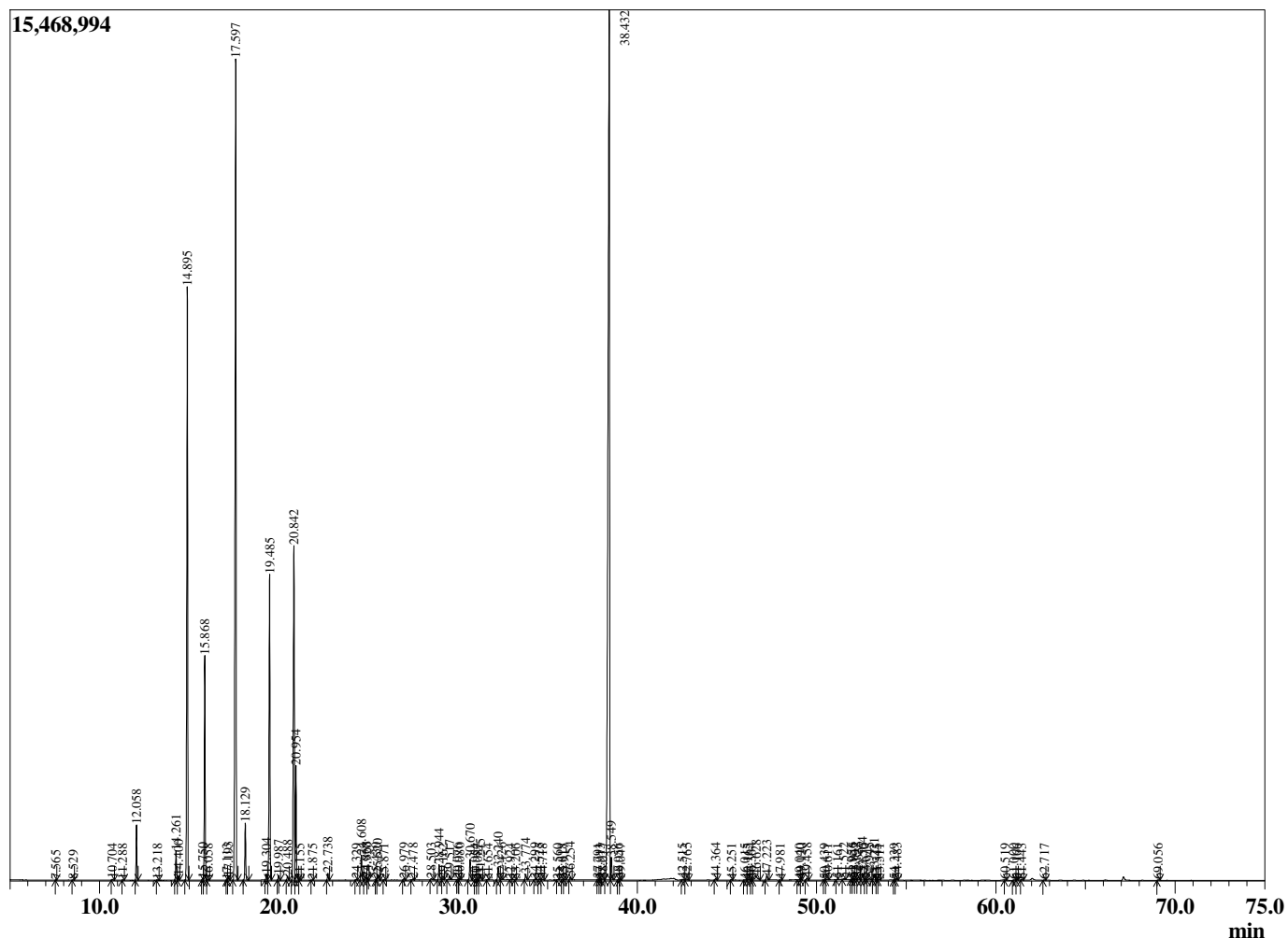
Chromatogram Tsuga canadensis
